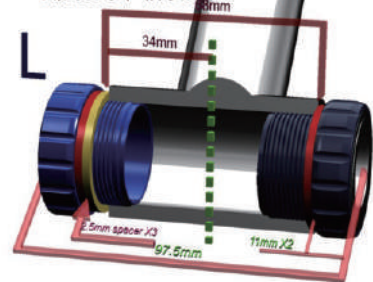
BB2495 (Thread type BOTTOM BRACKETS) (螺纹式中轴套)
