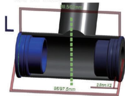
PFBB2492 (PRESS FIT ALLOY BOTTOM BRACKETS) (压入式中轴套)
