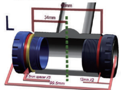
BB2497 (Thread type BOTTOM BRACKETS) (螺纹式中轴套)
