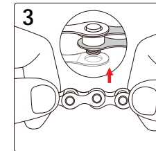
Place the Sigma top plate over the top of the free rivet groove while gently bending the Sigma link
